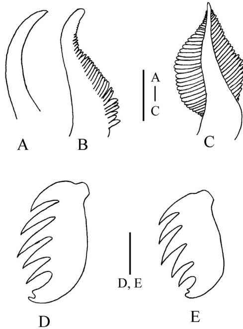
Figure 3. Phyllocomus chinensis sp. n. A awl-shaped branchiae from segment III B branchiae with one row of lamellae from segment II C branchiae with two rows of lamellae from segment 5 D thoracic uncinus from segment 7, lateral view; E abdominal uncinus from segment 20, lateral view. Scale bars A–C : 1 mm, D–E : 10 μm.
