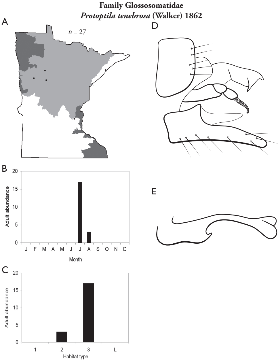
Figure 29. Protophila tenebrosa A total specimens collected and all known collecting localities (Figure 4) B monthly adult abundance (1980s to present) C habitat preference (1980s to present) (Table 1) D male genital capsule E phallus.
