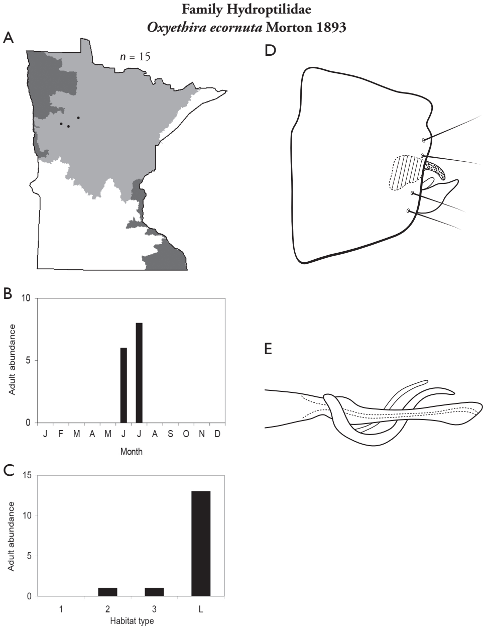
Figure 108. Oxyethira ecornuta A total specimens collected and all known collecting localities (Figure 4) B monthly adult abundance (1980s to present) C habitat preference (1980s to present) (Table 1) D male genital capsule E phallus.
