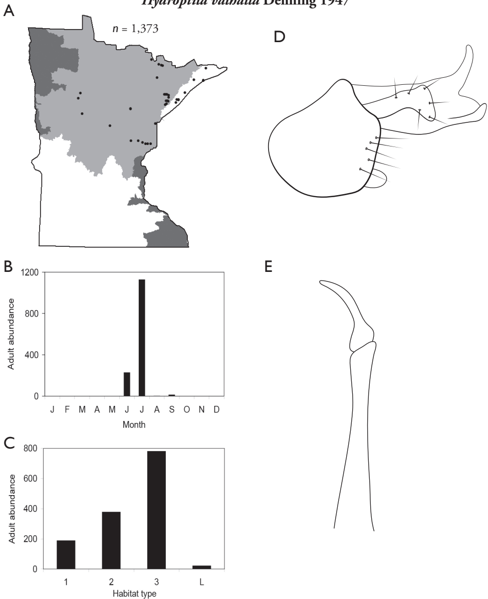
Figure 85. Hydroptila valhalla A total specimens collected and all known collecting localities (Figure 4) B monthly adult abundance (1980s to present) C habitat preference (1980s to present) (Table 1) D male genital capsule E phallus.
