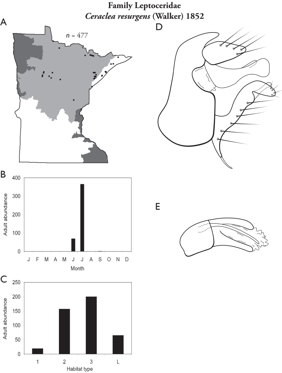
Figure 144. Ceraclea resurgens A total specimens collected and all known collecting localities (Figure 4) B monthly adult abundance (1980s to present) C habitat preference (1980s to present) (Table 1) D male genital capsule E phallus.
