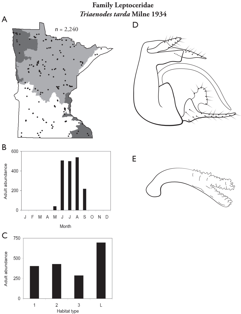
Figure 175. Trianenodes tarda A total specimens collected and all known collecting localities (Figure 4) B monthly adult abundance (1980s to present) C habitat preference (1980s to present) (Table 1) D male genital capsule E phallus.
