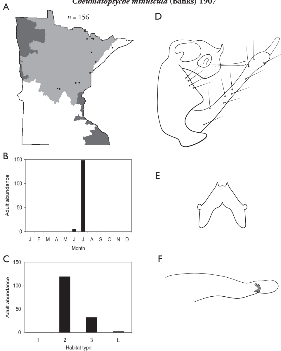
Figure 36. Cheumatopsyche miniscula A total specimens collected and all known collecting localities (Figure 4) B monthly adult abundance (1980s to present) C habitat preference (1980s to present) (Table 1) D male genital capsule E Lobes of tergum X (caudal view) F phallus.
