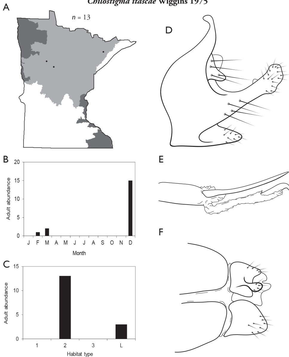
Figure 186. Chilostigma itasca A total specimens collected and all known collecting localities (Figure 4) B monthly adult abundance (1980s to present) C habitat preference (1980s to present) (Table 1) D male genital capsule E phallus F female genital capsule.
