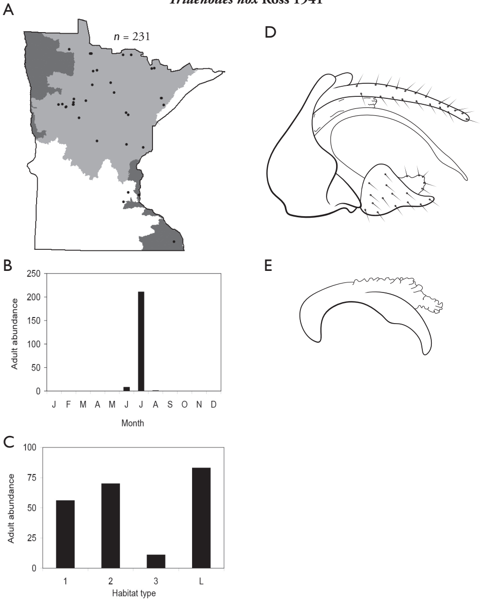
Figure 174. Triadenodes nox A total specimens collected and all known collecting localities (Figure 4) B monthly adult abundance (1980s to present) C habitat preference (1980s to present) (Table 1) D male genital capsule E phallus.
