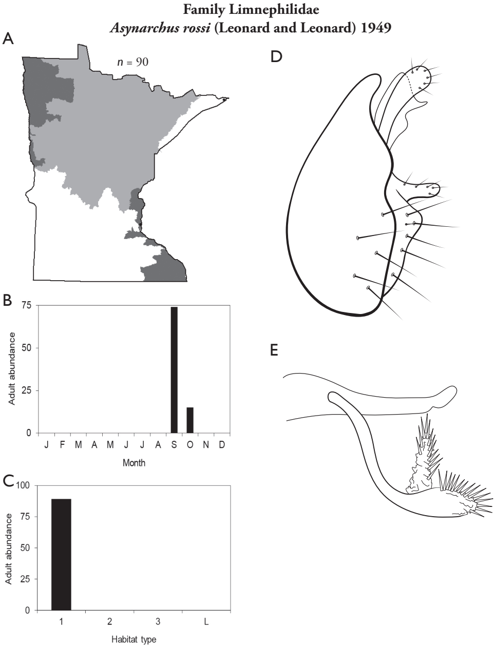
Figure 185. Asynarchus rossi A total specimens collected and all known collecting localities (Figure 4) B monthly adult abundance (1980s to present) C habitat preference (1980s to present) (Table 1) D male genital capsule E phallus.
