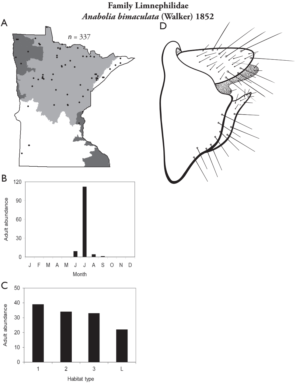
Figure 178. Anobolia bimaculata A total specimens collected and all known collecting localities (Figure 4) B monthly adult abundance (1980s to present) C habitat preference (1980s to present) (Table 1) D male genital capsule.
