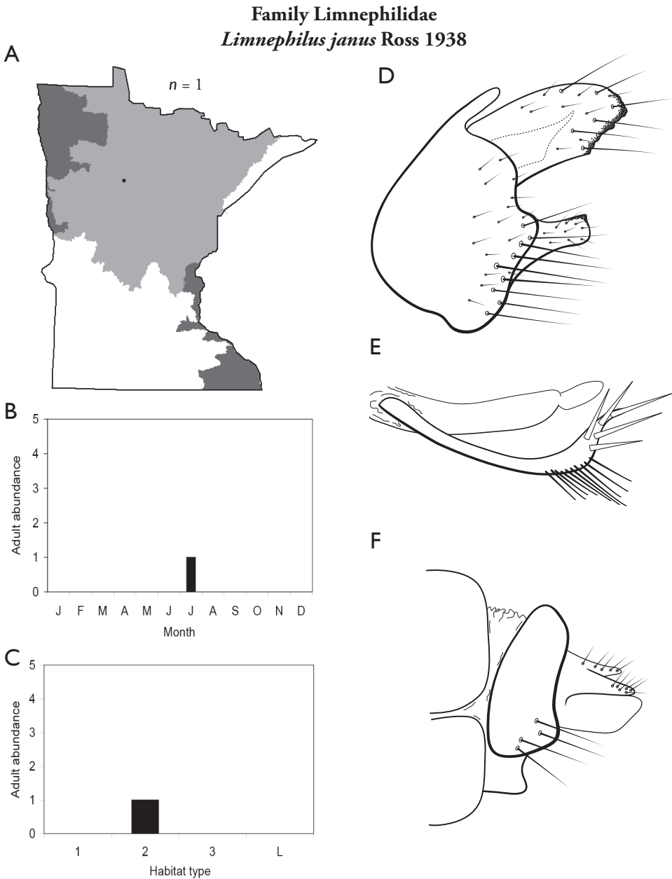
Figure 202. Limnephilus janus A total specimens collected and all known collecting localities (Figure 4) B monthly adult abundance (1980s to present) C habitat preference (1980s to present) (Table 1) D male genital capsule E phallus F female genital capsule.
