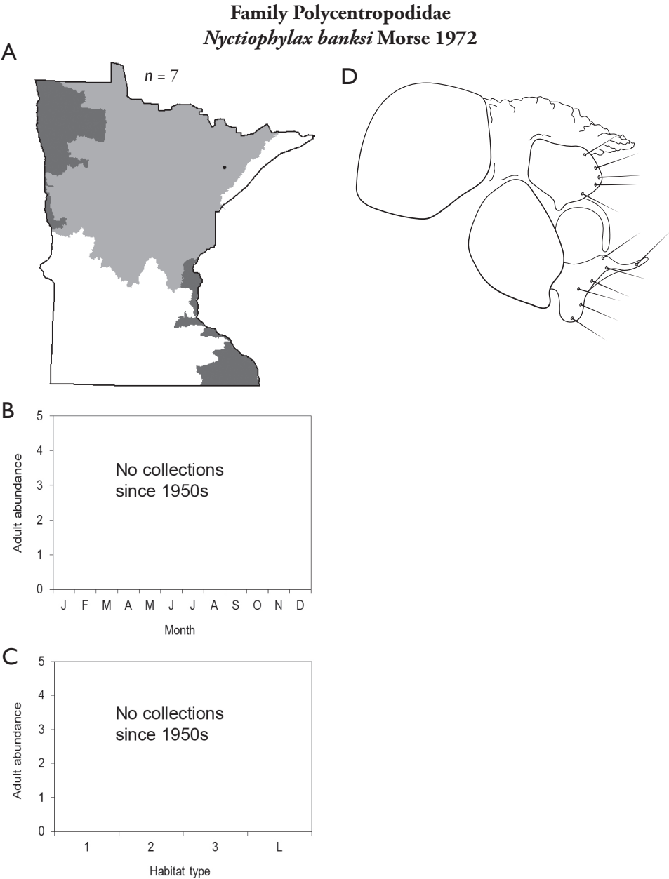
Figure 261. Nyctiophylax banksi A total specimens collected and all known collecting localities (Figure 4) B monthly adult abundance (1980s to present) C habitat preference (1980s to present) (Table 1) D male genital capsule.
