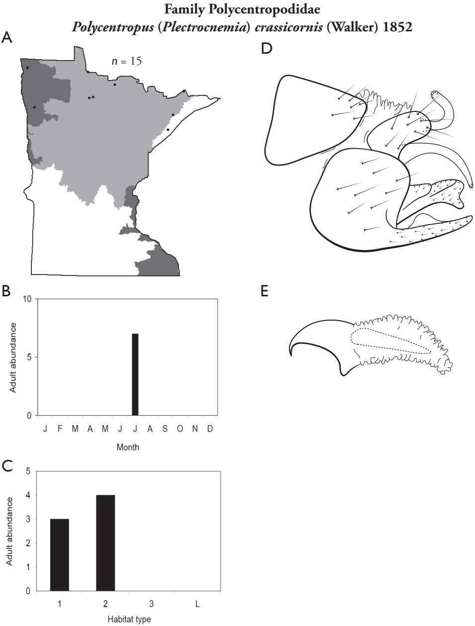
Figure 270. Polycentropus crassicornis A total specimens collected and all known collecting localities (Figure 4) B monthly adult abundance (1980s to present) C habitat preference (1980s to present) (Table 1) D male genital capsule E phallus.
