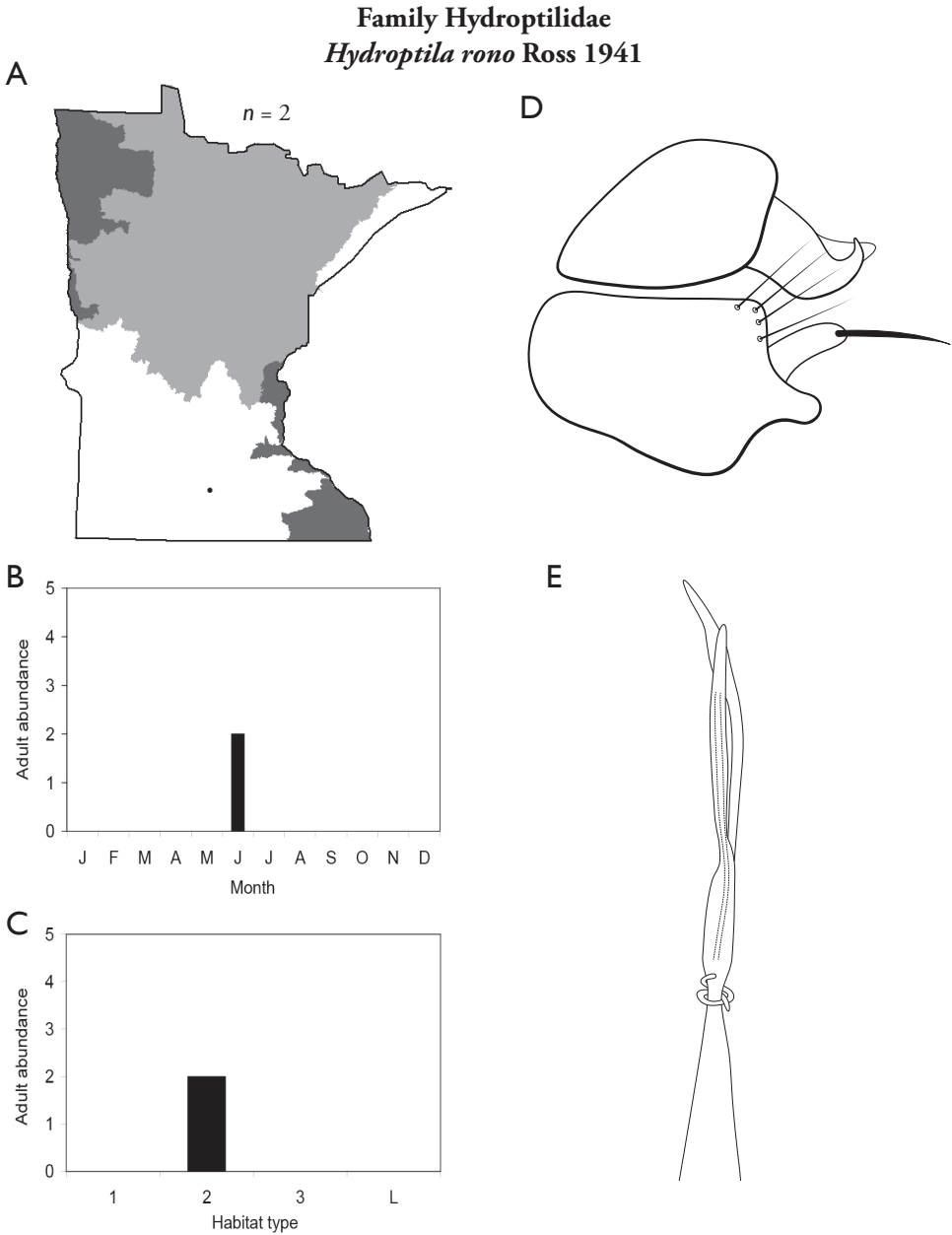
Figure 81. Hydroptila rono A total specimens collected and all known collecting localities (Figure 4) B monthly adult abundance (1980s to present) C habitat preference (1980s to present) (Table 1) D male genital capsule E phallus.
