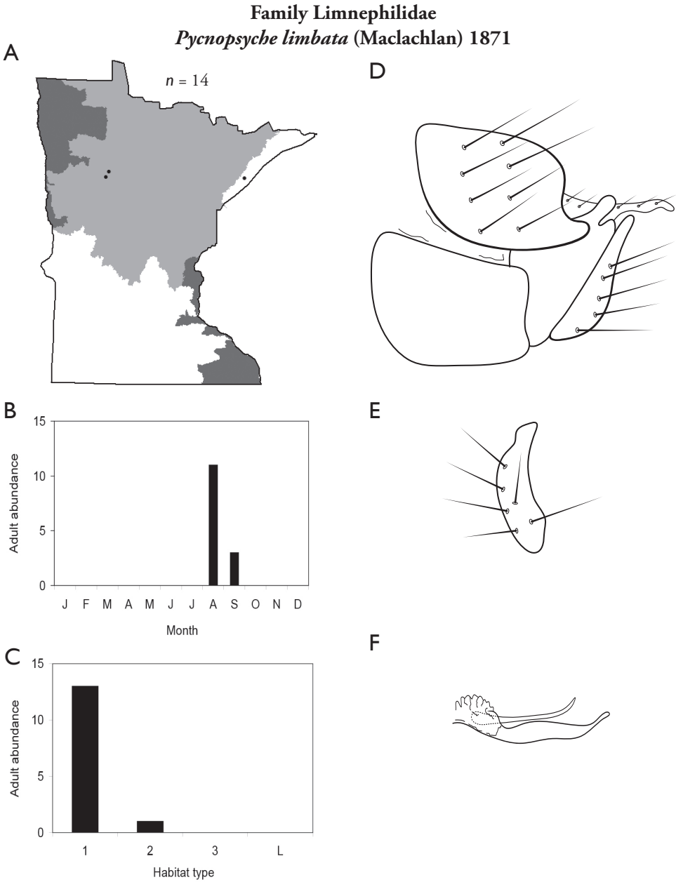
Figure 225. Pycnopsyche limbata A total specimens collected and all known collecting localities (Figure 4) B monthly adult abundance (1980s to present) C habitat preference (1980s to present) (Table 1) D male genital capsule E male inferior appendage (caudal view) F phallus.
