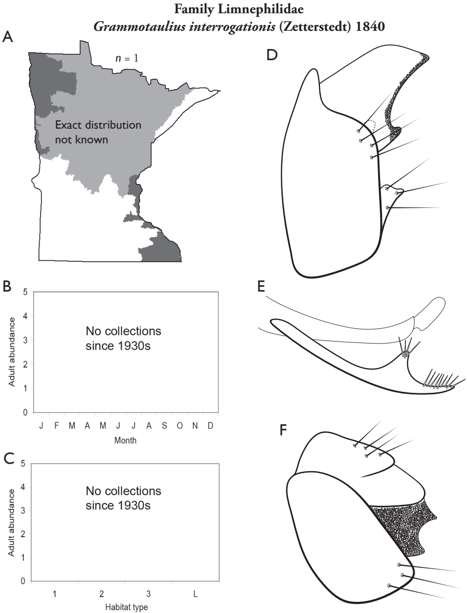
Figure 189. Grammotaulius interrogationis A total specimens collected and all known collecting localities (Figure 4) B monthly adult abundance (1980s to present) C habitat preference (1980s to present) (Table 1) D male genital capsule E phallus F female genital capsule.
