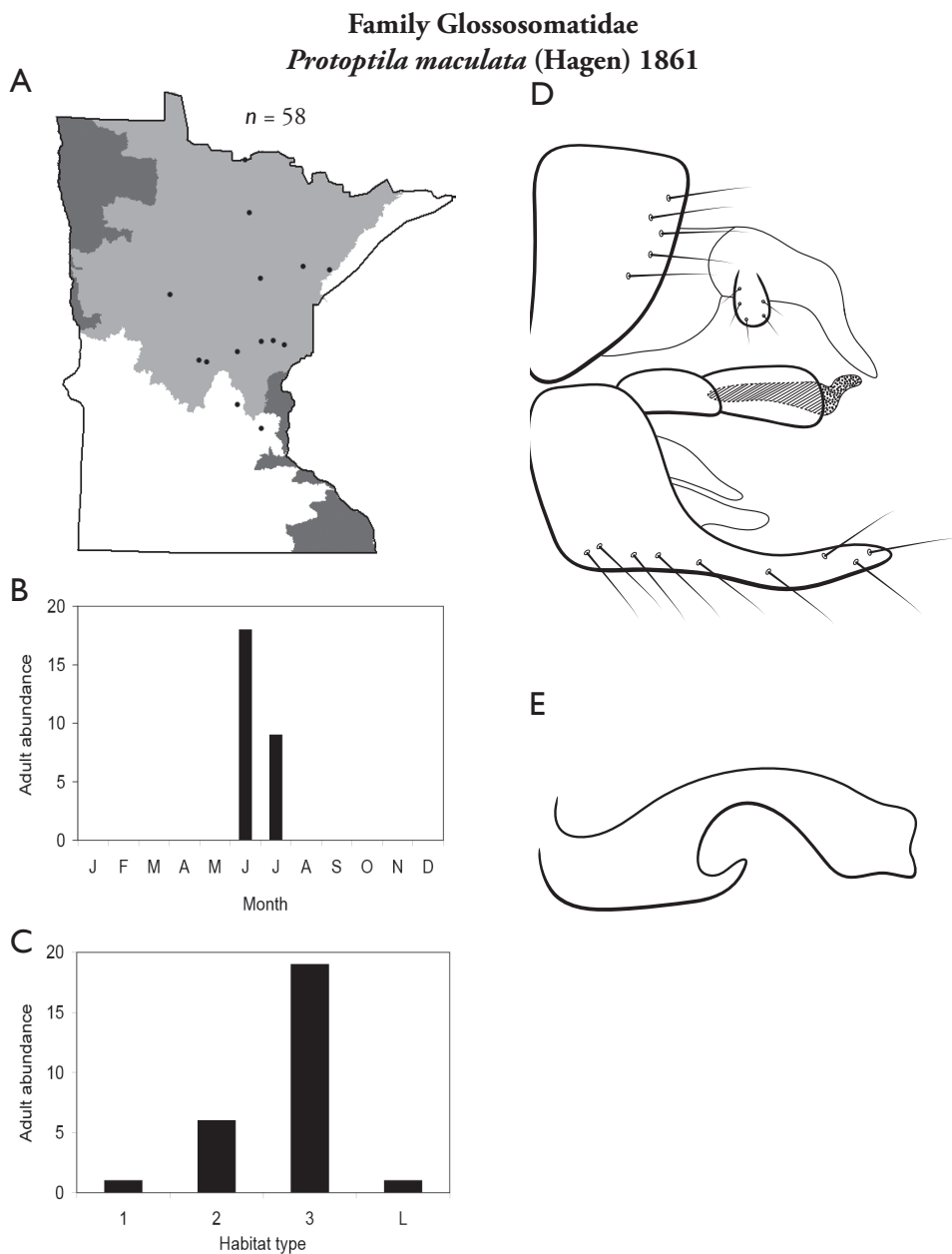
Figure 28. Protophila maculata A total specimens collected and all known collecting localities (Figure 4) B monthly adult abundance (1980s to present) C habitat preference (1980s to present) (Table 1) D male genital capsule E phallus.
