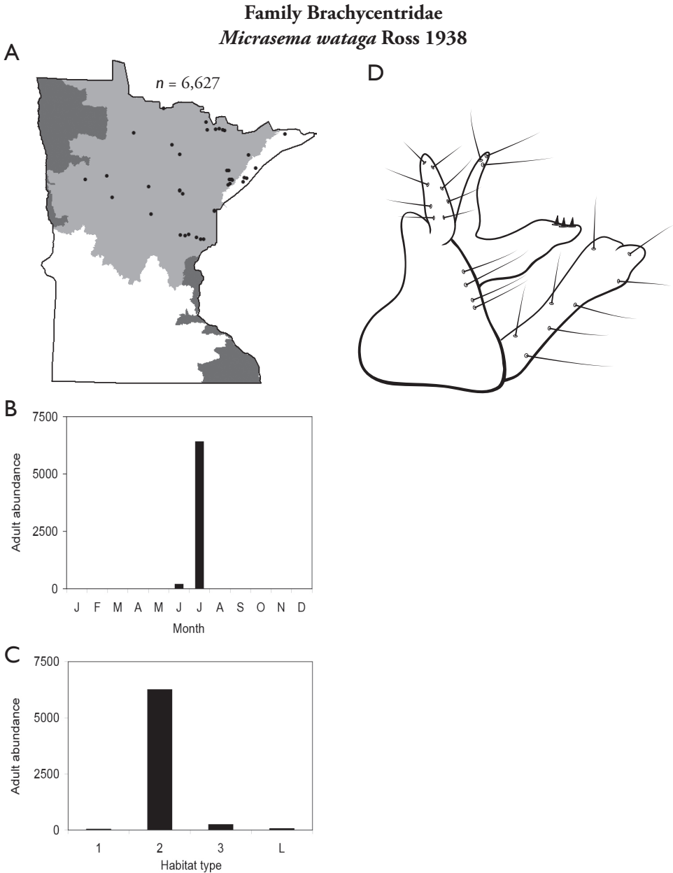
Figure 21. Micrasema wataga A total specimens collected and all known collecting localities (Figure 4) B monthly adult abundance (1980s to present) C habitat preference (1980s to present) (Table 1) D male genital capsule.
