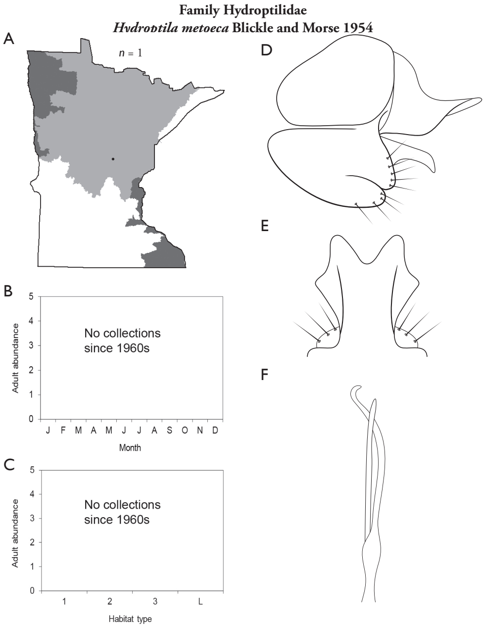
Figure 77. Hydroptila metoea A total specimens collected and all known collecting localities (Figure 4) B monthly adult abundance (1980s to present) C habitat preference (1980s to present) (Table 1) D male genital capsule E male genital capsule (ventral view) F phallus.
