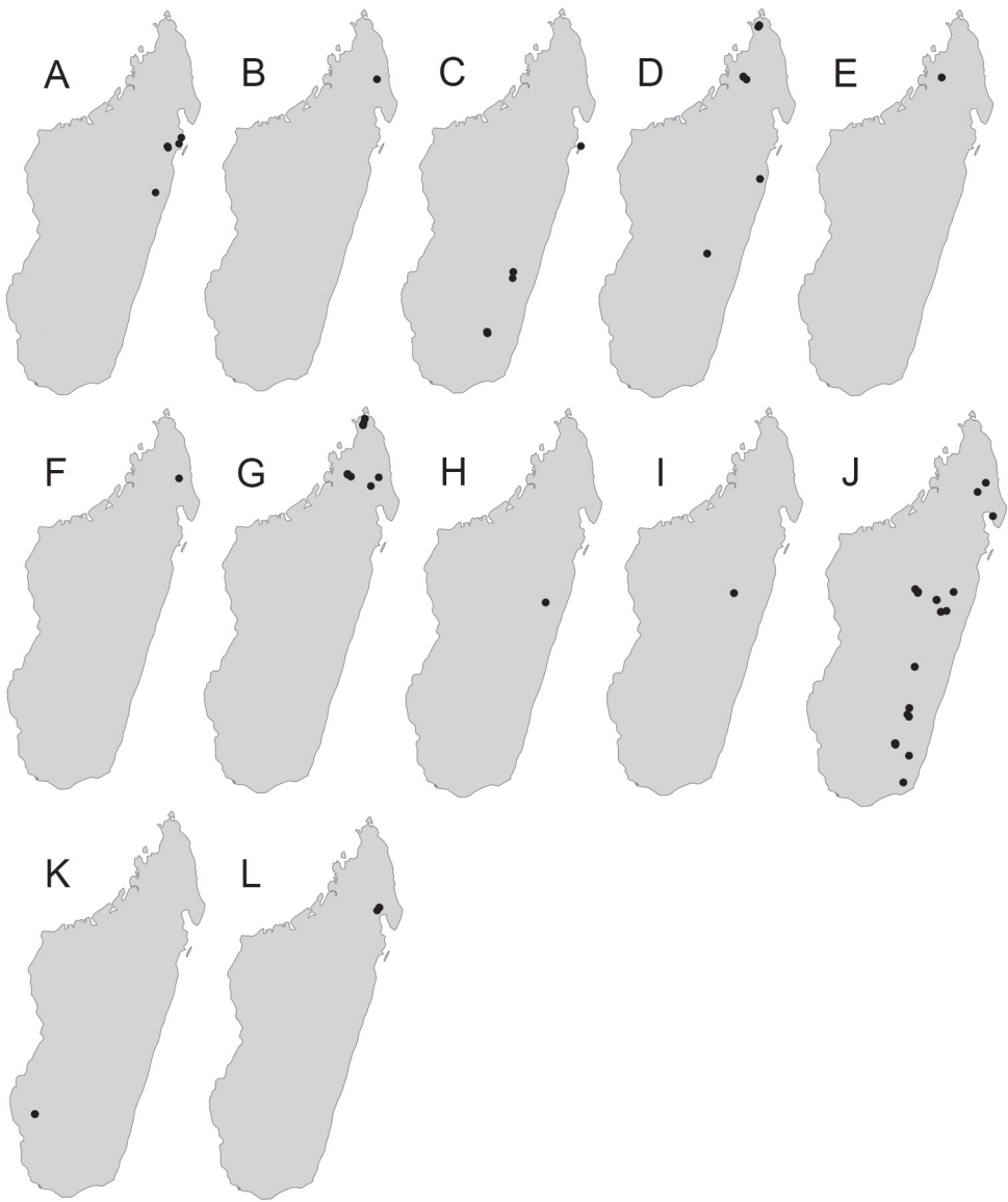
Figure 67. Distribution. Pheidole renirano sp. nov. (A). Pheidole sava sp. nov. (B). Pheidole sikorae Forel (C). Pheidole sofia sp. nov. (D). Pheidole sparsa sp. nov. (E). Pheidole tampony sp. nov. (F). Pheidole trichotos sp. nov. (G). Pheidole tsaravoniana sp. nov. (H). Pheidole vadum sp. nov. (I). Pheidole veteratrix Forel (J). Pheidole voluntany sp. nov. (K). Pheidole vony sp. nov. (L).
