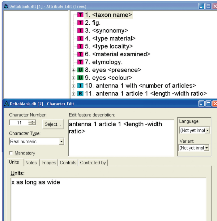
Figure 9a–b. Numeric character types. Examples of a Integer numeric b Real numeric .
