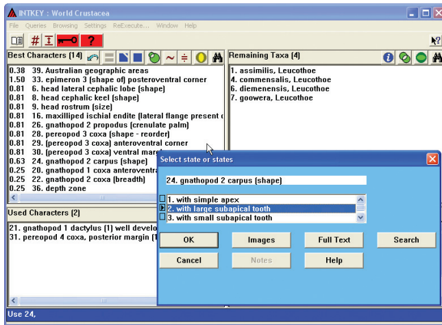
Figure 68. Character 24 again splits the Remaining Taxa into two equally large groups.
