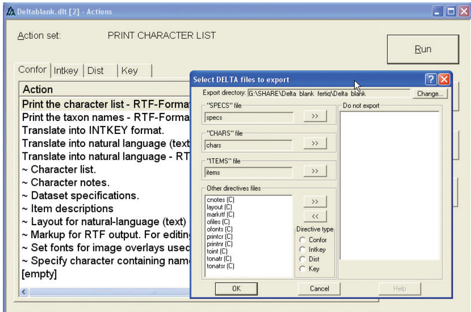
Figure 25. Confor in the DELTA Editor asks the user to make a selection of directive files being exported.
