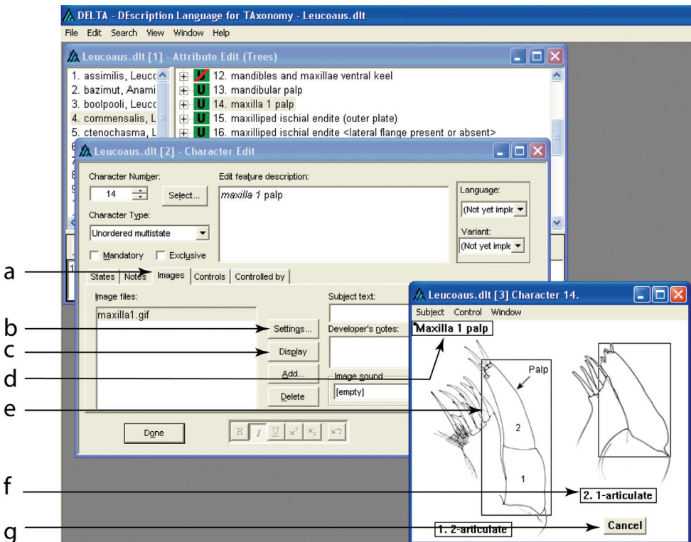
Figure 17a–g. Character state images. a the Images tab in the Character editor b Settings allow the selection of the path to the image directory and font details for the overlays c Display shows the selected image file in a window with the character and overlay boxes d feature text of the character e Hotspot selection box f character state overlay box g Cancel box. These overlays are used in Intkey.
