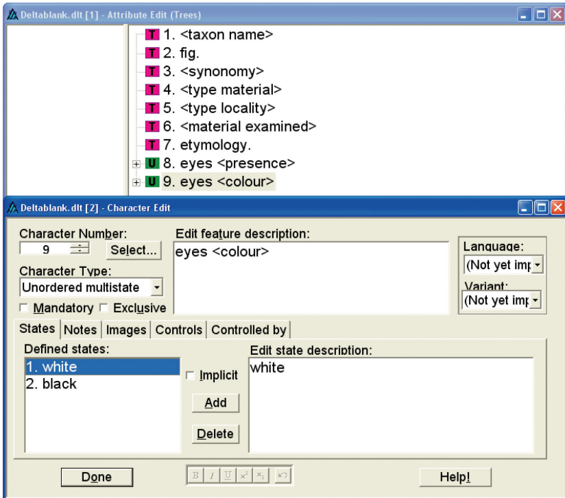
Figure 7a–b. Definition of two Unordered multistate characters.
