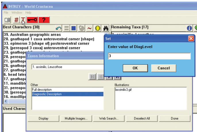
Figure 56. Raising the diagnostic level.
