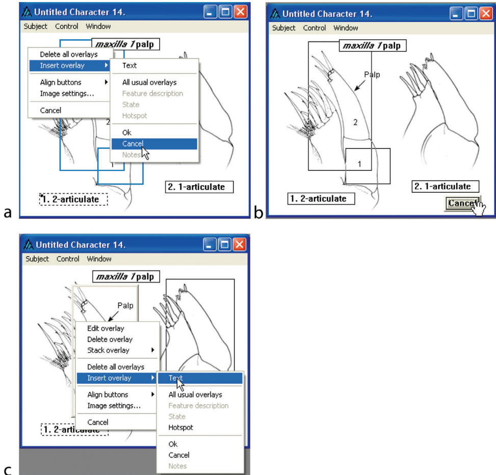
Figure 21. Inserting a Cancel button and additional text overlays on a character illustration.
