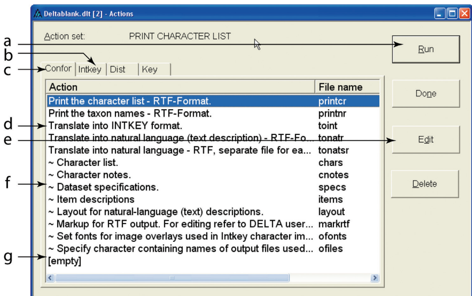
Figure 22a–g. The Confor dialog tab in Action sets.
