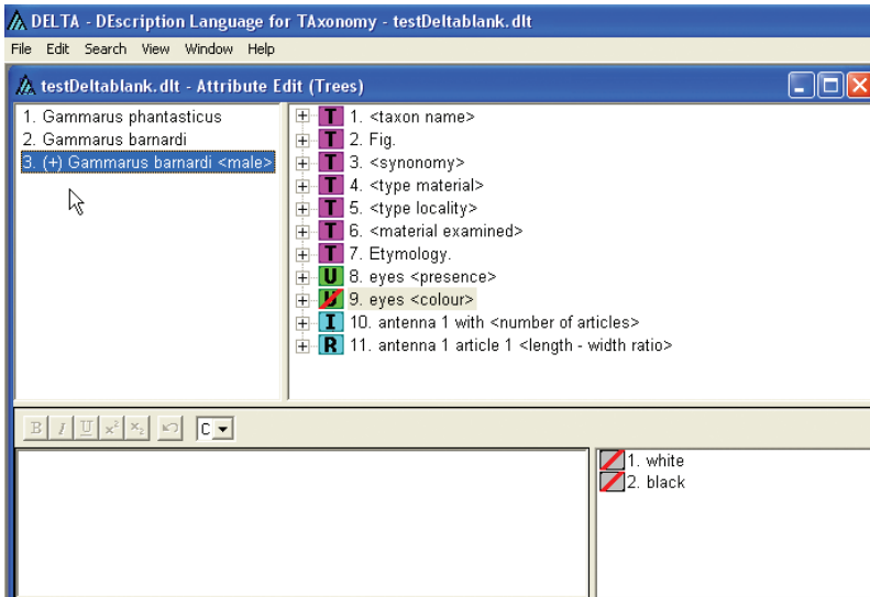
Figure 13. Inserting a taxon that was marked as a variant ( Treat as variant ) in the Taxon editor, indicated by (+) preceding the taxon name.
