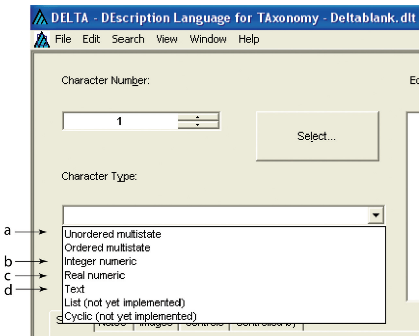
Figure 5a–d. Character types selection from the Character editor.
