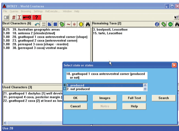
Figure 78. Character 20 is connected to character 18. Clicking on character 20 will open character 18 first.
