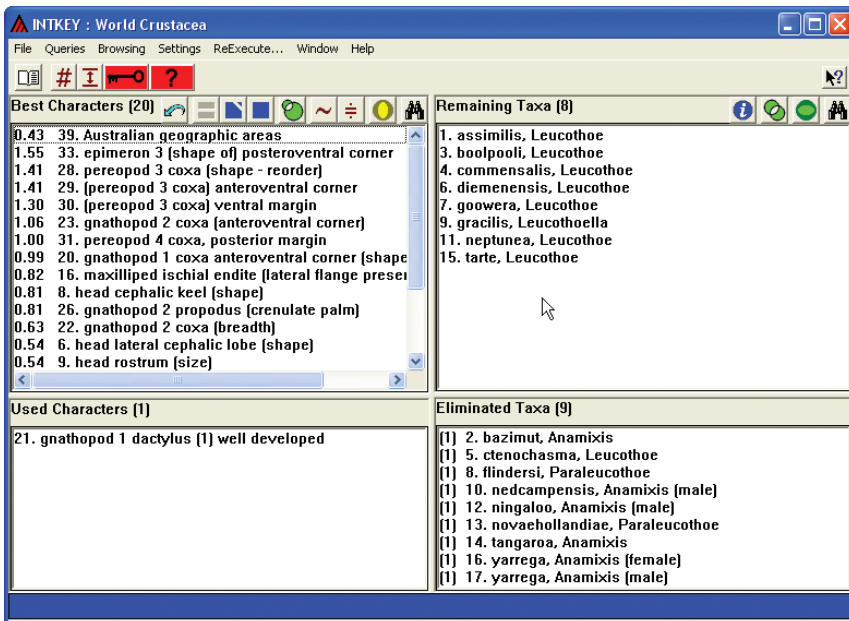
Figure 65. The first character separated the taxa into two groups of about equal size. For the Eliminated Taxa the selected character state did not match.
