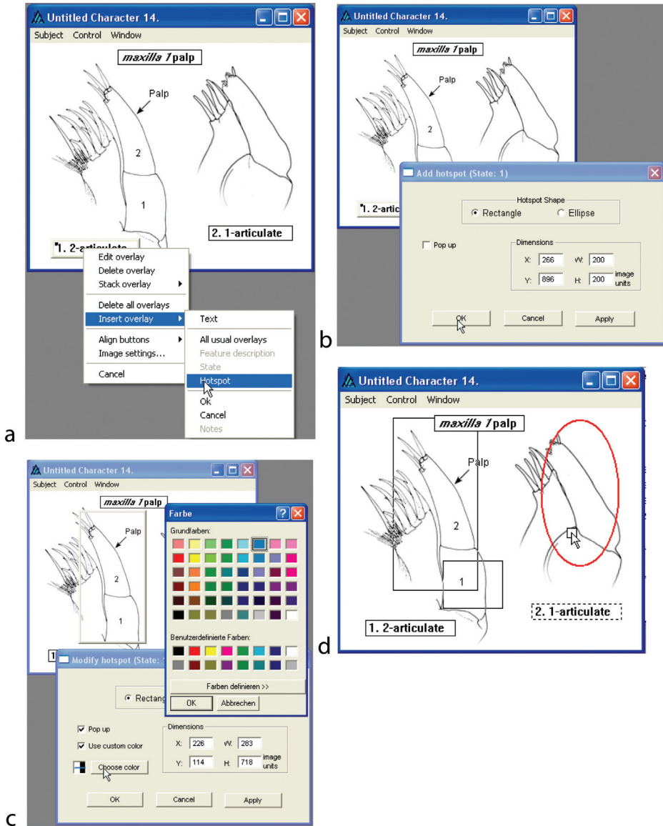
Figure 20a–d. Creating hotspots on a character image.
