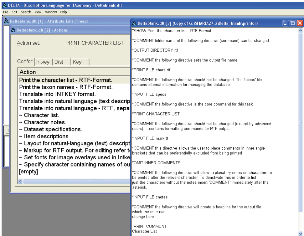
Figure 23. The Print the character list (printer) directive file was opened by pushing the Edit button.
