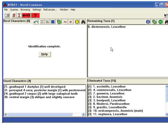
Figure 70. The identification sequence for one part of the key is complete. Now we go back a few steps to continue to work on the key.
