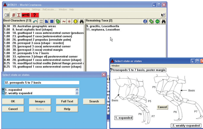
Figure 74. Clicking on the Images button during the selection of character states will show the illustrations for all character states.
