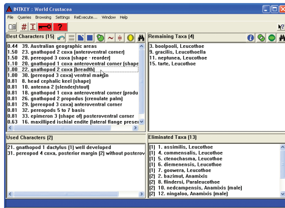
Figure 71. The second group of taxa is used to create the dichotomous key.
