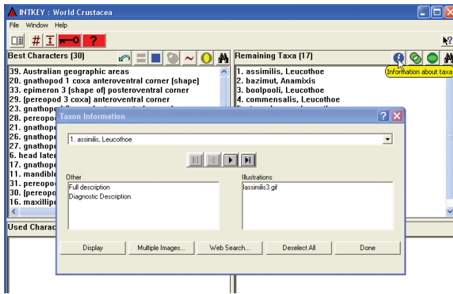
Figure 53. Information about taxa button.
