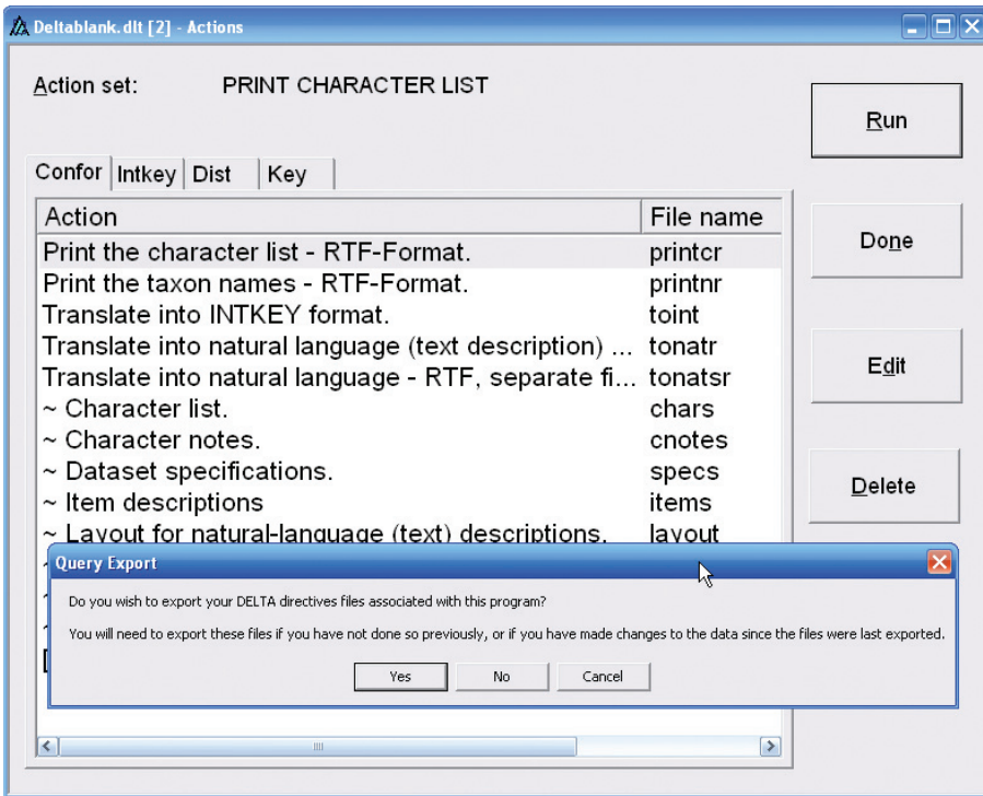
Figure 24. When running a directive file the program asks for an export of the directive files.
