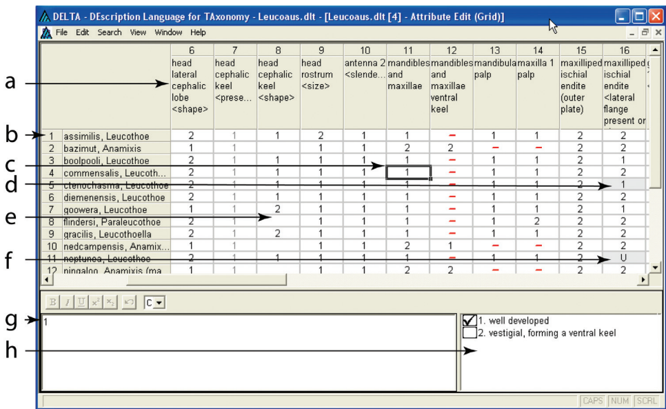
Figure 14a–h. Attribute editor in the Grid view. a character feature text b taxon list c selection box shows character state 1 selected. The red dash of character 12 indicates that this character is inapplicable d the grey background in the box indicates that a comment in angle brackets was made to specify the character state e unrecorded character f character states explicitly marked unknown g character state pane, where aside from the input of the character state as a number comments can be made in angle brackets h character state selection check boxes.
