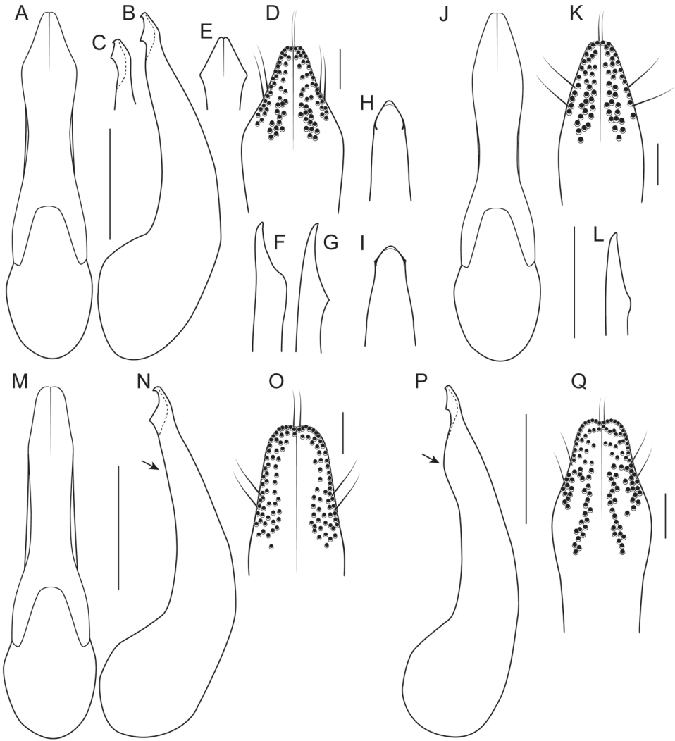
Figure 8. Bolitogyrus electus Smetana & Zheng ( A, B, D, F, H ), B. uncus Cai et al. ( C, E, G, I ), B. confusus Brunke ( J–L ), B. huangbaoi Hu et al. ( M–O ) and B. nigropolitus Smetana ( P, Q ). Aedeagus in parameral view ( A, J, M ), median lobe in lateral view ( B, C, N, P ), peg setae of paramere ( D, K, O, Q ), apex of paramere in lateral ( F, G, L ) and parameral view ( E ), apex of median lobe in parameral view ( H, I ). Figure 8E modified from Cai et al. (2015). Scale bars: 0.5 mm ( A–C, E–J, L–N, P ), 0.1 mm ( D, K, O, Q ).
