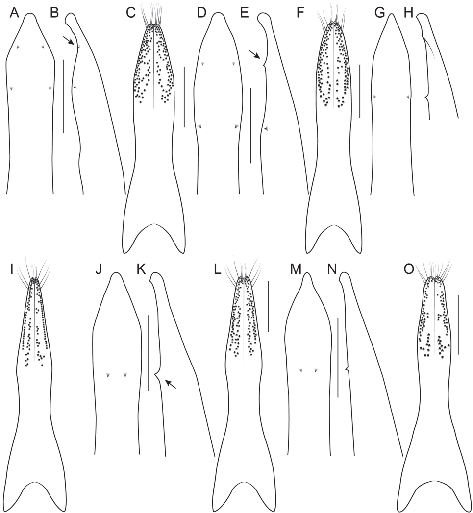
Figure 11. Bolitogyrus carnifex (Fauvel) (A–C), B. pedersenii Brunke (D–F), B. vietnamensis (Scheerpeltz) (G–I), B. elegantulus Yuan et al. (J–L) and B. phukhieo Brunke (M–O). Median lobe in parameral view (A, D, G, J, M), median lobe in lateral view (B, E, H, K, N), peg setae of paramere (C, F, I, L, O). Scale bars: 0.5 mm.
