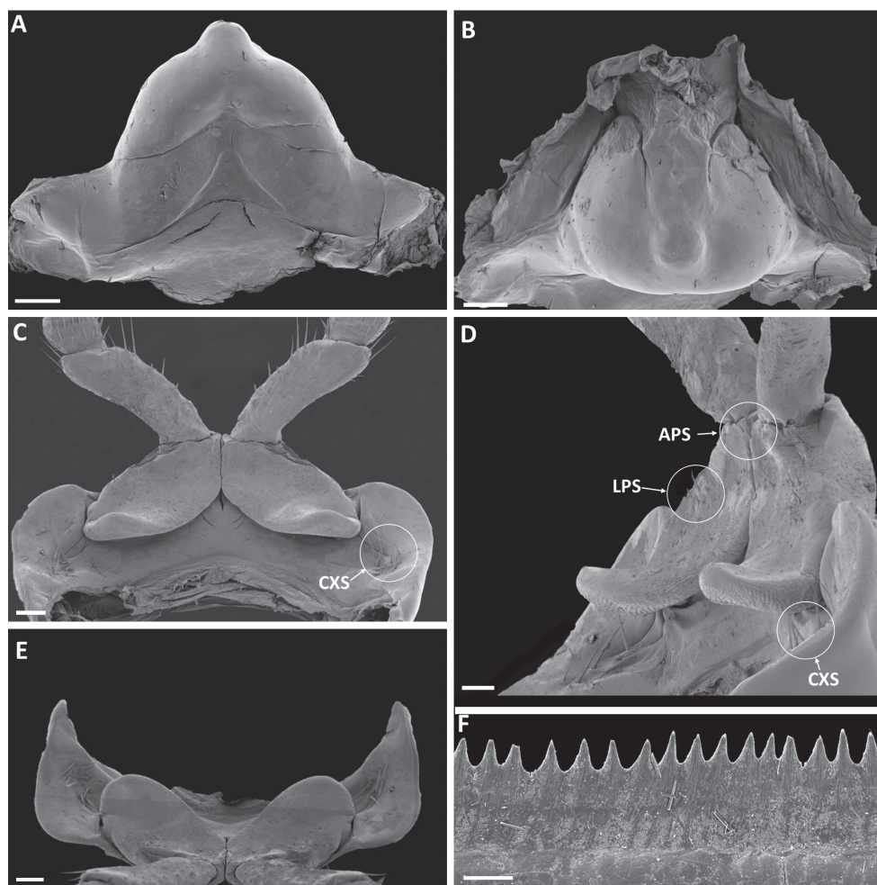
Figure 2. Pleonoporus tanzanicus sp. nov., paratype, ♂ (NHMD 621850) A, B sternum 9 A anterior view B ventral view C–E first pair of legs C anterior view D sublateral view E ventral view F limbus. Abbreviations: APS = mesapical prefemoral setae; CXS = coxosternal setae; LPS = lateral prefemoral setae. Scale bars: 0.2 mm ( A–E ); 0.02 mm ( F ).
