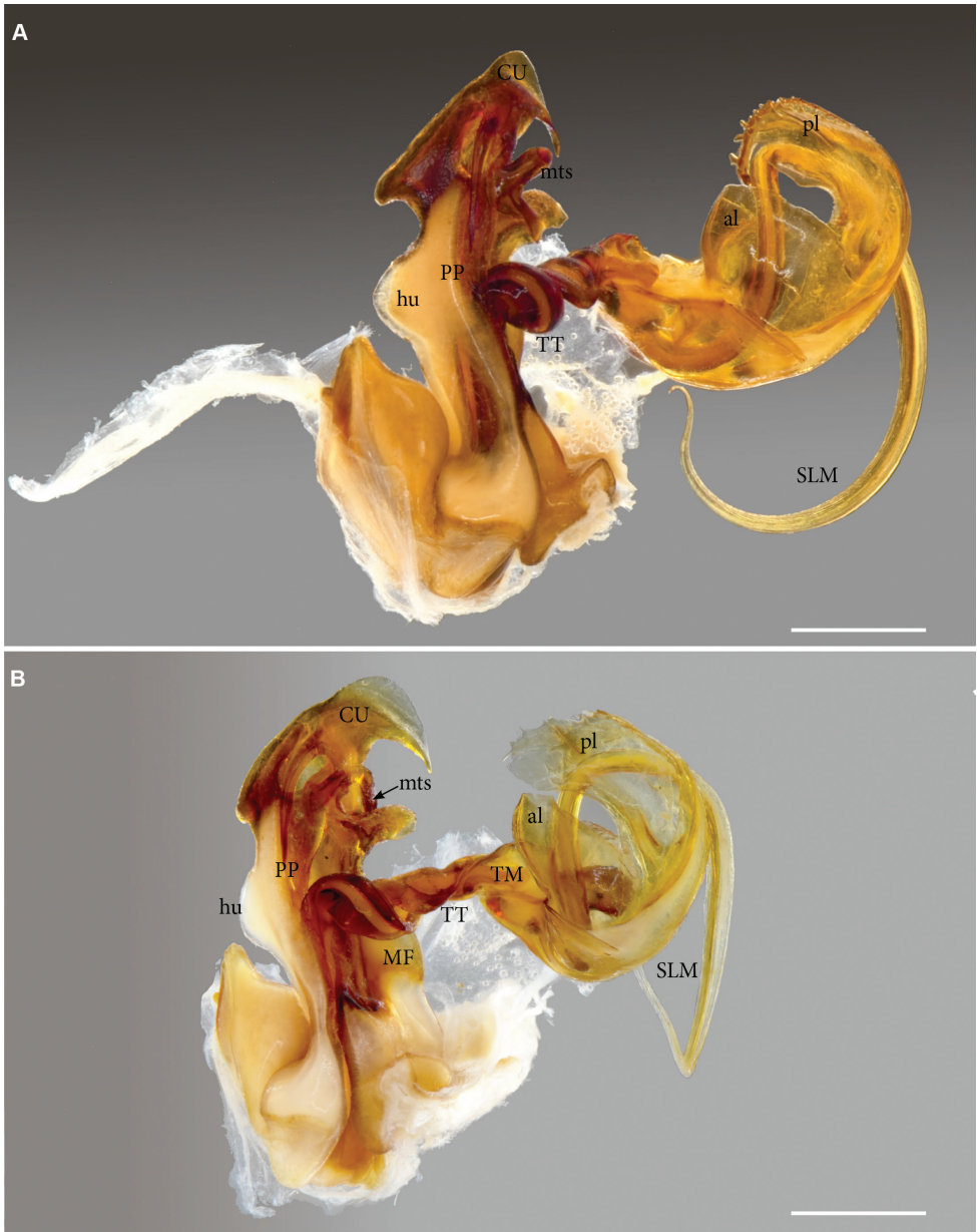
Figure 7. Pleonoporus robustus Attems, 1938. Syntype ♂ gonopods (NHMW MY 9062) A right gonopod, anterior view B antero-mesal view. Abbreviations: al = anterior lobe of telomere, CU = cucullus; hu = lateral hump; MF = metaplical flange, MP = metaplica; msp = metaplical spine; mts = metaplical transverse spine; PP = proplica; pl = posterior lobe of telomere, SLM = solenomere; TM = telomere; TT = torsotope. Scale bars: 1 mm.
