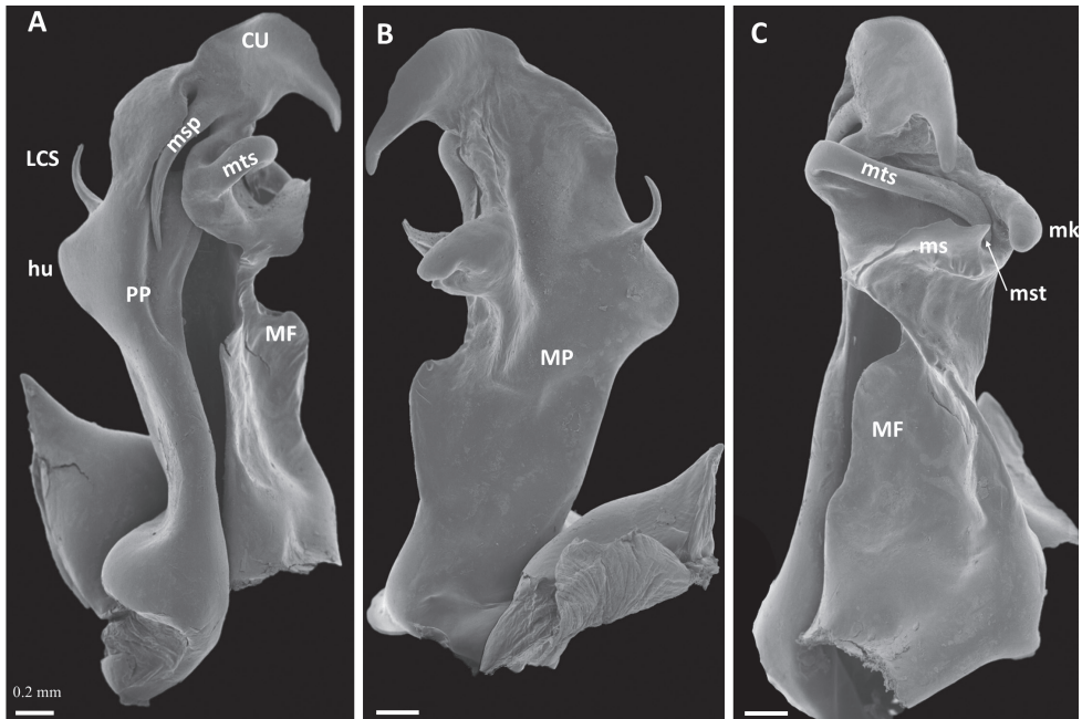
Figure 3. Pleonoporus tanzanicus sp. nov., paratype, ♂ (NHMD 621850), left gonopod coxa A anterior view B posterior view C mesal view. Abbreviations: CU = cucullus; hu = lateral hump; LCS = lateral coxal spine; MF = metaplical flange; mk = metaplical knob; MP = metaplica; ms = metaplical shelf; msp = metaplical spine; mst = metaplical shelf tooth; mts = metaplical transverse spine; PP = proplica. Scale bars: 0.2 mm.
