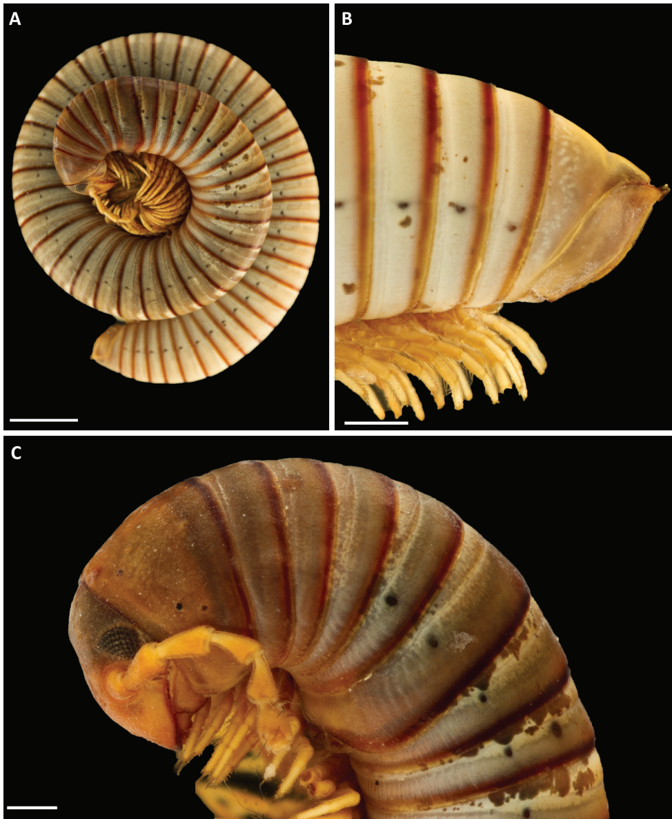
Figure 1. Pleonoporus tanzanicus sp. nov. A paratype ♂, habitus (ZMH ZMH-0016676) B holotype ♂ (ZMH-0016675) Last four body rings and telson C paratype ♂, head and first nine body rings (NHMW MY10277). Scale bars: 5 mm ( A ); 1 mm ( B , C ).
