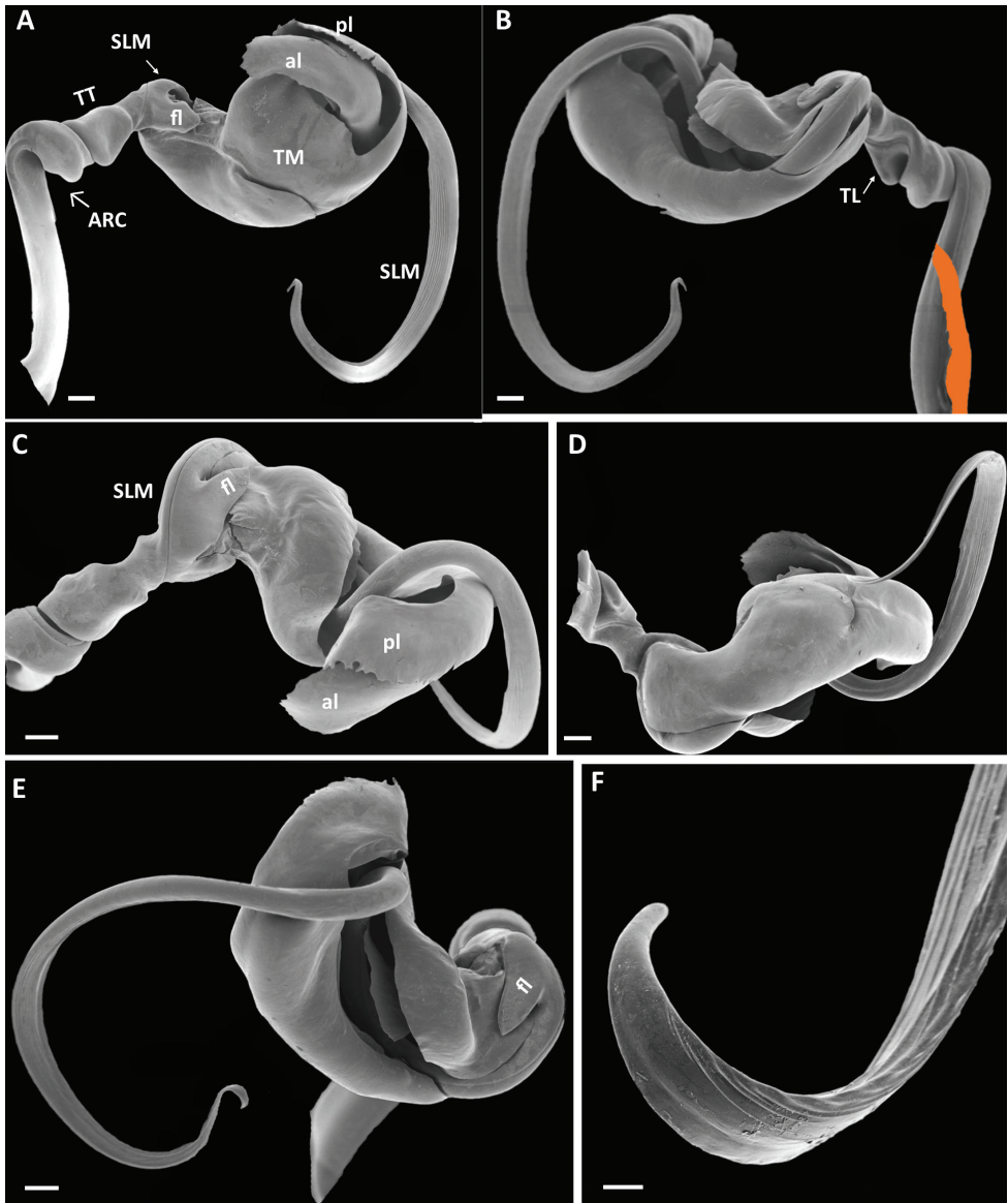
Figure 4. Pleonoporus tanzanicus sp. n., paratype, ♂ (NHMD 621850), left gonopod telopodite A anterior view B posterior view (basomere partly covered by mounting tape (orange)) C ventral (apical) view D basal (dorsal) view E mesal view F tip of solenomere. Abbreviations: al = anterior lobe of telomere; ARC = arculus; fl = basal flap of solenomere; pl = posterior lobe of telomere; SLM = solenomere; TL = torsotope lobe; TM = telomere; TT = torsotope. Scale bars: 0.2 mm ( A–E ); 0.02 mm ( F ).
