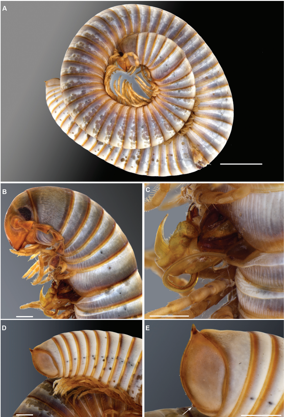
Figure 5. Pleonoporus robustus Attems, 1938. Syntype ♂ (NHMW MY 2666) A male, in toto lateral view B head and anteriormost rings, lateral view C close-up of gonopod in situ, lateral view D posterior-most rings and telson, lateral view E close-up of the telson, arrow indicating ventral projections. Scale bars: 5 mm ( A ); 1 mm ( B–D ).
