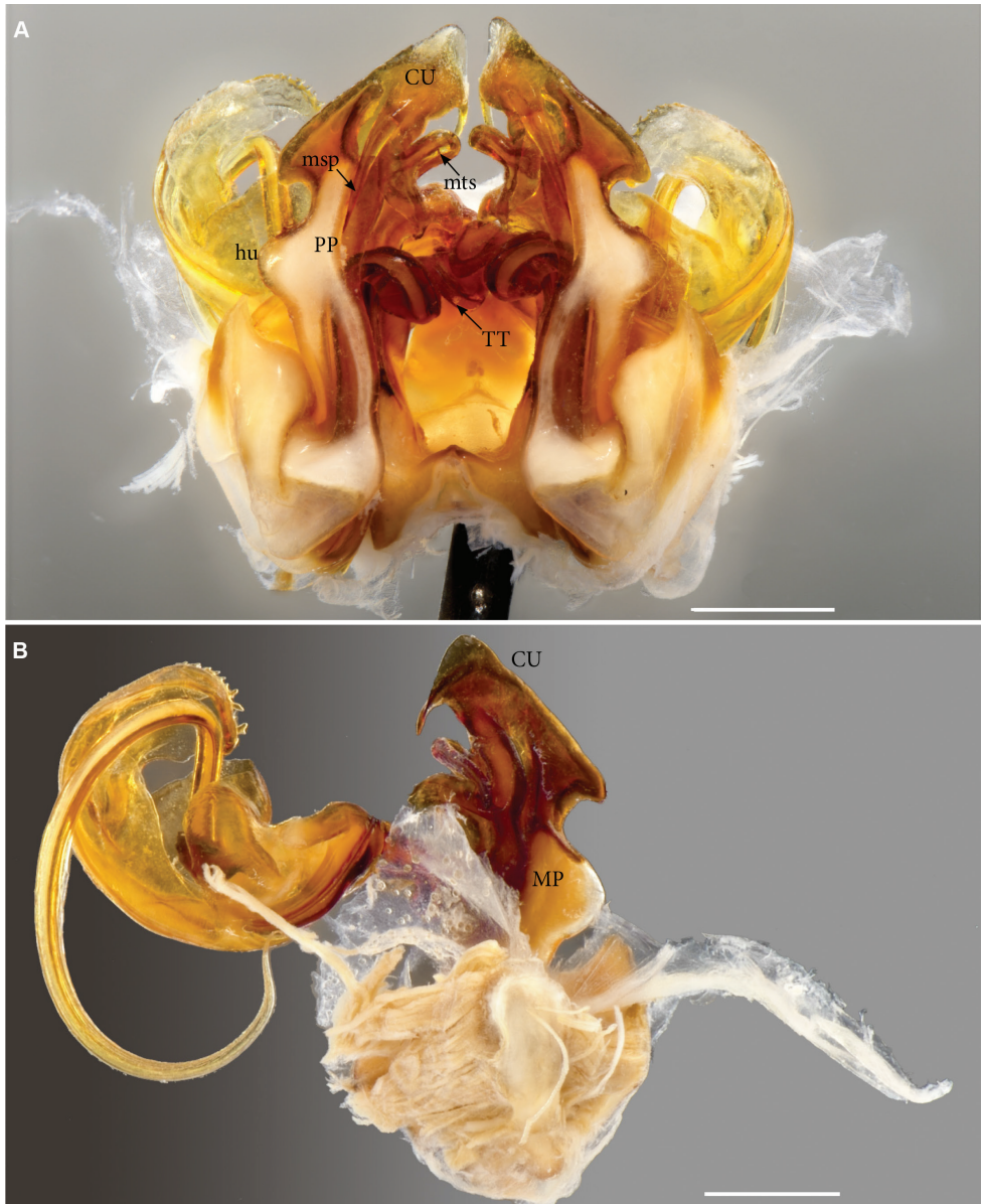
Figure 6. Pleonoporus robustus Attems, 1938. Syntypes ♂ gonopods A gonopod block (NHMW MY9061), anterior view B left gonopod, posterior view (NHMW MY 9062). Abbreviations: CU = cucullus; hu = lateral hump; MP = metaplica; msp = metaplical spine; mts = metaplical transverse spine; PP = proplica; Scale bars: 1 mm.
