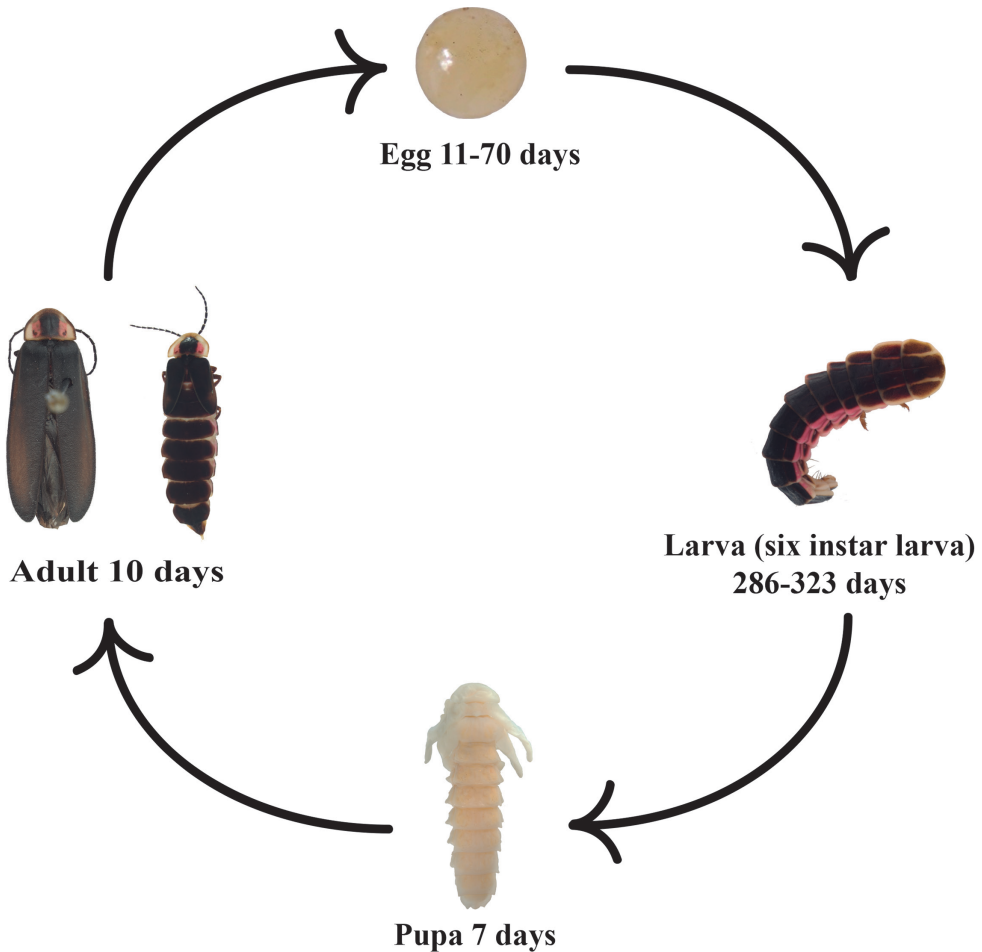
Figure 11. Life cycle of Photinus extensus Gorham.
