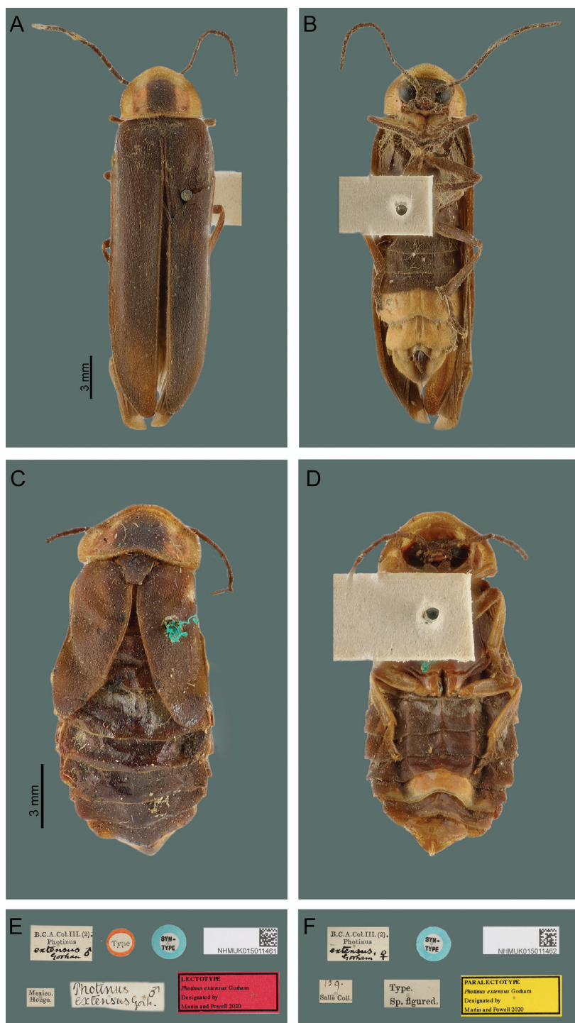
Figure 2. Photinus extensus Gorham, type specimens NHM-London A general habitus of the adult male in dorsal view B ventral view C general habitus of the adult female in dorsal view D ventral view E male labels (lectotype) F female labels (paralectotype). Photos: Keita Matsumoto.
