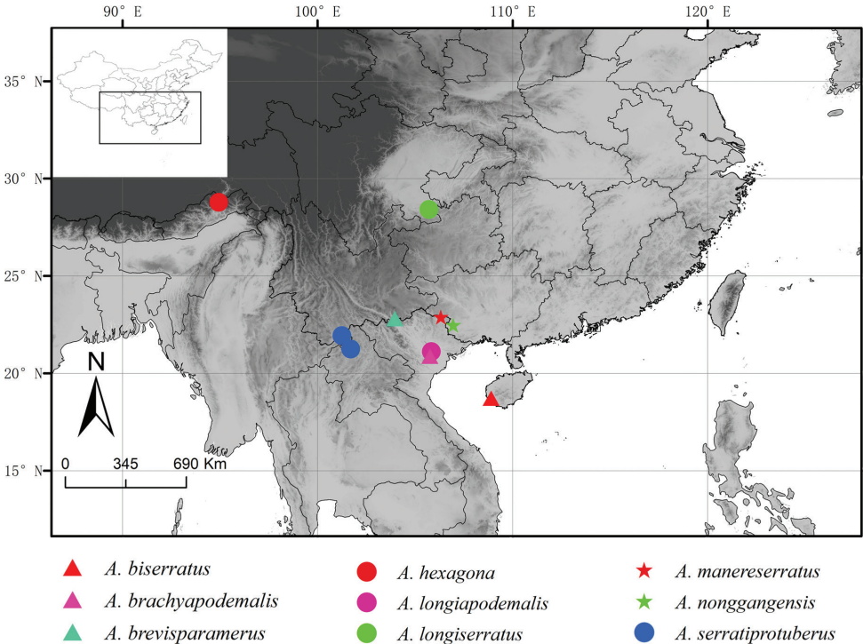
Figure 1. Known distribution of Anaxiphomorpha species, including the new species A. nonggangensis sp. nov. and A. manereserratus sp. nov..
