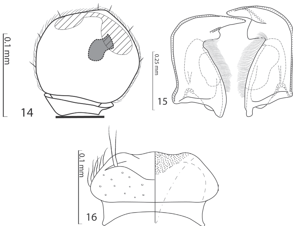
Figure 14–16. 14 Exaesiopus grossipes (Marseul, 1855) sensory structures of the antenna 15 mandibles, dorsal view 16 labrum, left half depicting dorsum; right half depicting underside.
