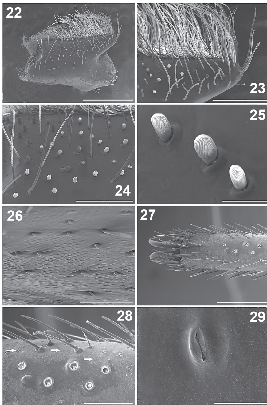
Figures 22–29. Paratropis tuxtlensis sp. n. Male. 22 Left endite, dorsal view 23 Left endite, apical detail 24 Left endite, detail of the setae 25 Detail of the finger-shaped cuspules on endite 26 Detail of the setae on retrolateral region of left endite 27 Left leg I, dorsal view of the tarsus 28 Left tarsus I, detail of the trichobothria sockets (arrows indicate the cuticular pores) 29 Detail of the glandular pore on the surface of the tarsus. Scales: 10 \mu m (Figure 29), 50 \mu m (Figure 25), 100 \mu m (Figure 26), 200 \mu m (Figure 28), 300 \mu m (Figure 24), 400 \mu m (Figure 23), 500 \mu m (Figure 27), 1 mm (Figure 22).
