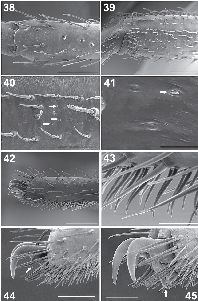
Figures 38–45. Paratropis tuxtlensis sp. n. Male. 38 Left leg, trichobothria of metatarsus I, dorsal view 39 Left leg, setae on tibia I, retrolateral view 40 Detail of setae on tibiae I (arrows indicate the glandular pores) 41 Detail of the glandular pores on tibia I (arrow indicates pore with secretion) 42 Left leg, tarsus I, retrolateral view 43 Detail of the scopular setae on tarsus I 44 Claws of tarsus I, retrolateral view (arrow indicates the single long tooth on left claw) 45 Detail of the paired claws of tarsus I (arrow indicates the unpaired ventral claw). Scales: 40 \mu m (Figure 41), 100 \mu m (Figure 43), 200 \mu m (Figures 40, 45), 300 \mu m (Figure 44), 400 \mu m (Figure 38), 500 \mu m (Figures 39, 42).
