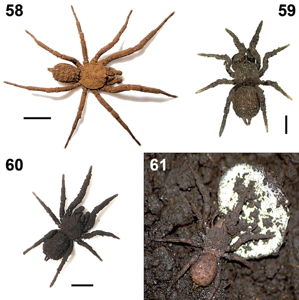
Figures 58–61. Paratropis tuxtlensis sp. n. Photographs of live specimens, kept in the laboratory 58 Adult male 59 Immature specimen 60 Adult female 61 Adult female protecting her egg sac. Scales: 1 mm (Figure 59), 4 mm (Figure 58), 6 mm (Figure 60).
