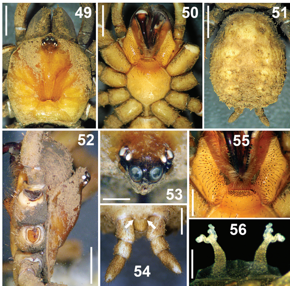
Figures 49–56. Paratropis tuxtlensis sp. n. Female. 49 Carapace, dorsal view 50 Prosoma, ventral view, showing the sternum, labium, endites and chelicerae 51 Opisthosoma, dorsal view 52 Carapace, left lateral view 53 Ocular region, dorsal view 54 Spinnerets, ventral view (arrows indicate the PMS) 55 Endites and labium, ventral view 56 Spermathecae, dorsal view. Scales: 0.25 mm (Figure 56), 0.6 mm (Figure 53), 1 mm (Figures 54, 55), 2 mm (Figures 49–52).
