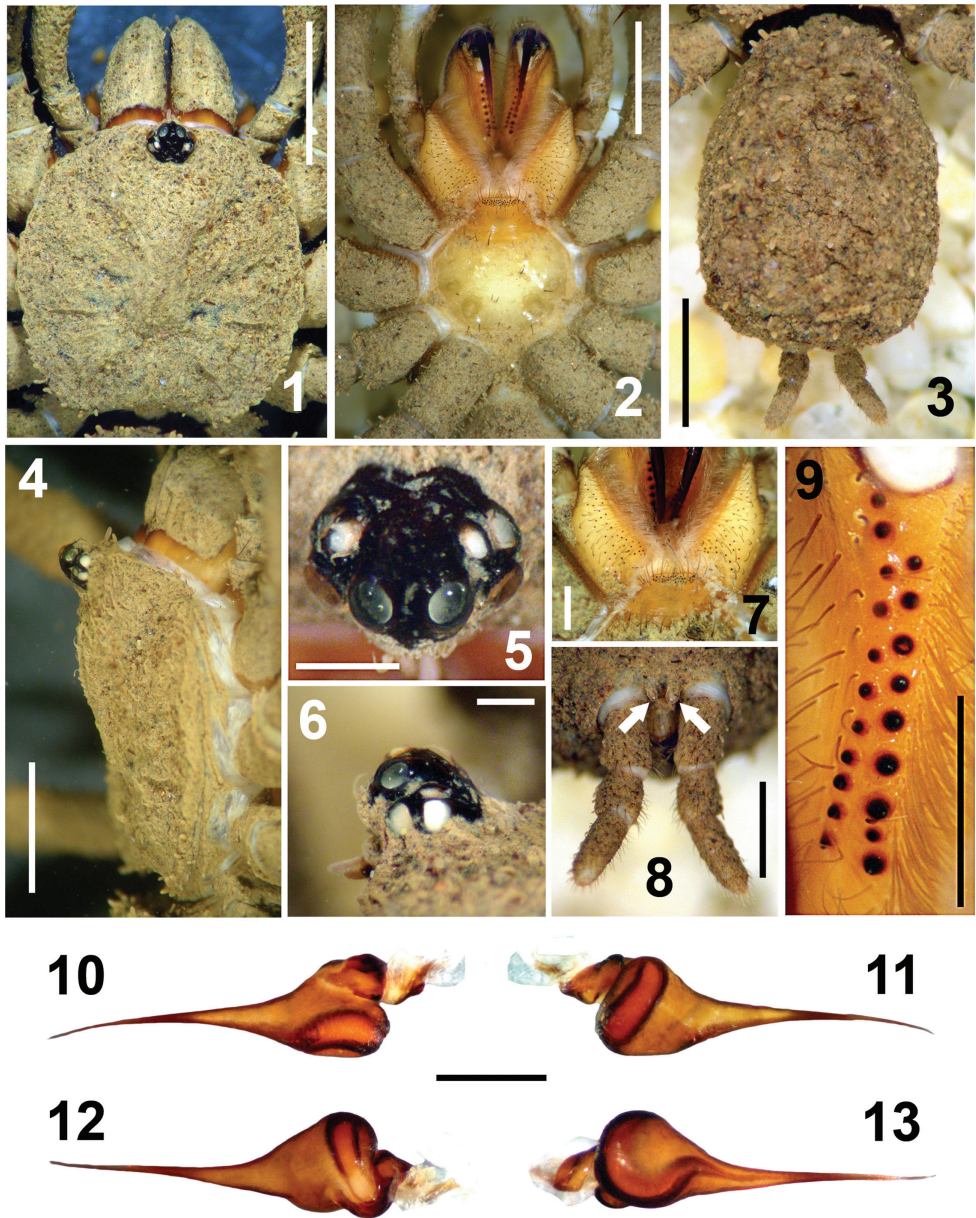
Figures 1–13. Paratropis tuxtensis sp. n. Male. 1 Carapace, dorsal view 2 Prosoma, ventral view, showing the sternum, labium, endites and chelicerae 3 Opisthosoma, dorsal view 4 Carapace, right lateral view 5–6 Ocular region, dorsal and lateral views, respectively 7 Endites and labium, ventral view 8 Spinnerets, ventral view (arrows indicate the PMS) 9 Left chelicerae, teeth on promargin (left) and retromargin (right) 10–13 Bulb and embolus, prolateral, retrolateral, dorsal, and ventral views respectively. Scales: 0.4 mm (Figures 5, 6), 0.5 mm (Figures 7, 9–13), 1 mm (Figure 8), 2 mm (Figures 1–4).
