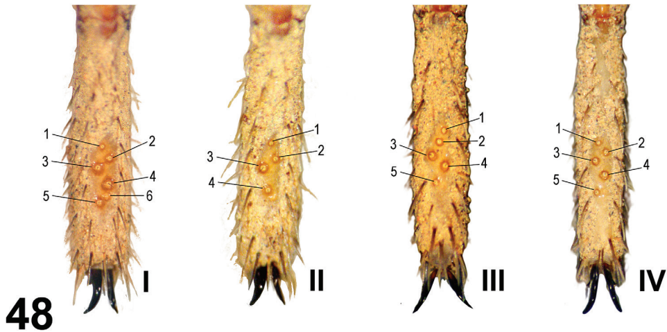
Figures 48. Paratropis tuxtensis sp. n. Trichobothria pattern on tarsi I–IV on male legs.
