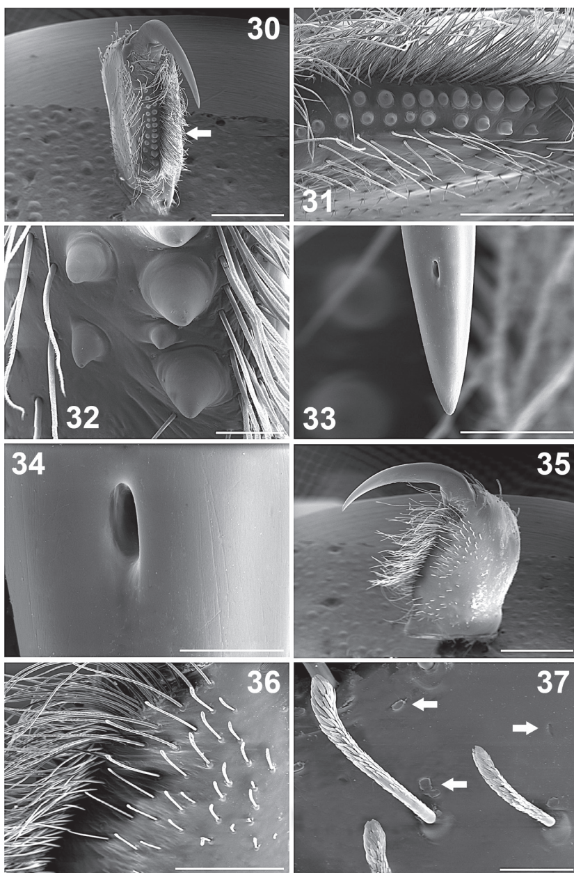
Figures 30–37. Paratropis tuxtlenensis sp. n. Male. 30 Left chelicerae with extended fang, ventral view 31 Left chelicerae, teeth on promargin (lower line) and retromargin (upper line) 32 Detail of the chelicerae teeth 33 Left chelicerae, apical part of the fang 34 Detail of the venom gland duct opening on left fang of the chelicerae 35 Left chelicerae, retrolateral view 36 Setae on retrolateral part of left chelicerae 37 Detail of the clubbed setae on retrolateral region of chelicerae (left arrows indicate the glandular pores on the cuticle surface with secretion coming out at the moment of the microphotograph, right arrow indicates pore without secretion). Scales: 20 \mu\text{m} (Figure 34), 50 \mu\text{m} (Figure 37), 100 \mu\text{m} (Figures 32, 33), 400 \mu\text{m} (Figure 36), 500 \mu\text{m} (Figure 31), 1 mm (Figures 30, 35).
