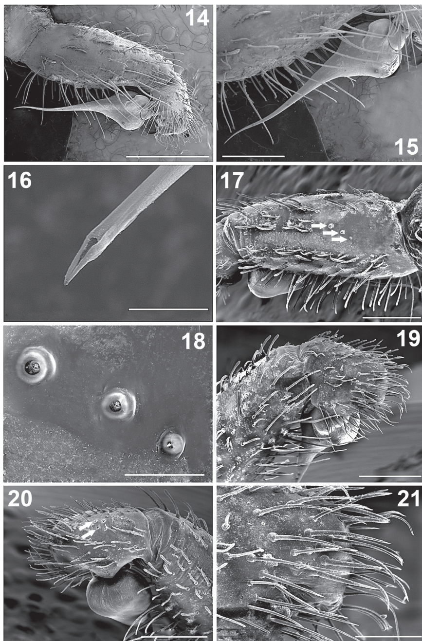
Figures 14–21. Paratropis tuxtlensis sp. n.. Male 14 Left palp, prolateral view 15 Left palp, detail of bulb and embolus, prolateral view 16 Detail of the embolus opening, distal view 17 Left palp tibia, dorsal-retrolateral view (arrows indicate the trichobothria) 18 Detail of the trichobothria sockets on the palp tibia 19 Left palp, tibia and tarsus, prolateral view 20 Left palp, tibia and tarsus, retrolateral view (arrows indicate the trichobothria) 21 Detail of the setae on tarsus of left palp, prolateral view. Scales: 10 \mu m (Figure 16), 100 \mu m (Figure 18), 200 \mu m (Figure 21), 500 \mu m (Figures 15, 17, 19, 20), 1 mm (Figure 14).
