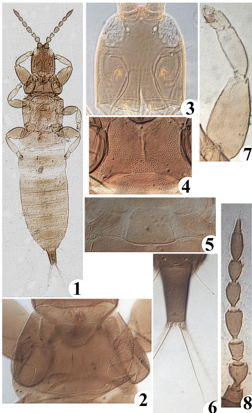
Figures 1–8. Karnyothrips cyathomorphus sp. n. 1 slide mounted apterous adult (dorsal view), female 2 pronotum, female 3 head, female 4 basantra and ferna, female 5 pelta, female 6 abdominal tergum IX and tube, male 7 fore leg, male 8 antenna, female.
